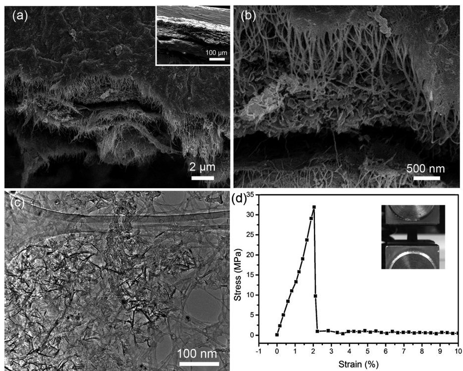
Figure 2. a) Cross-sectional and b) corresponding magnified SEM, and c) TEM images of the interconnected structure formed by the CoS 2 /RGO composite and CNTs. The inset indicates the thickness of the composite film. d) Typical stress–strain curve for the CoS 2 /RGO-CNT composite film.
