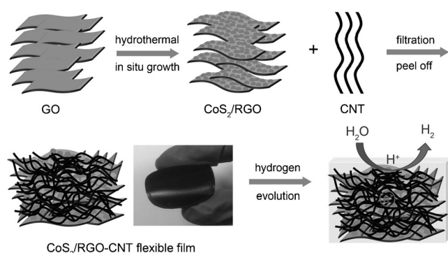
Scheme 1. Fabrication procedure and hydrogen evolution process of the freestanding CoS 2 /RGO-CNT hybrid electrode.
